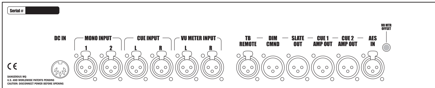
DANGEROUS MQ REAR PANEL
